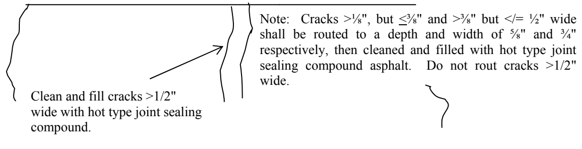
FIGURE 835-5: SEALING ASPHALT PAVEMENT CRACKS (>1/8" < 2")
