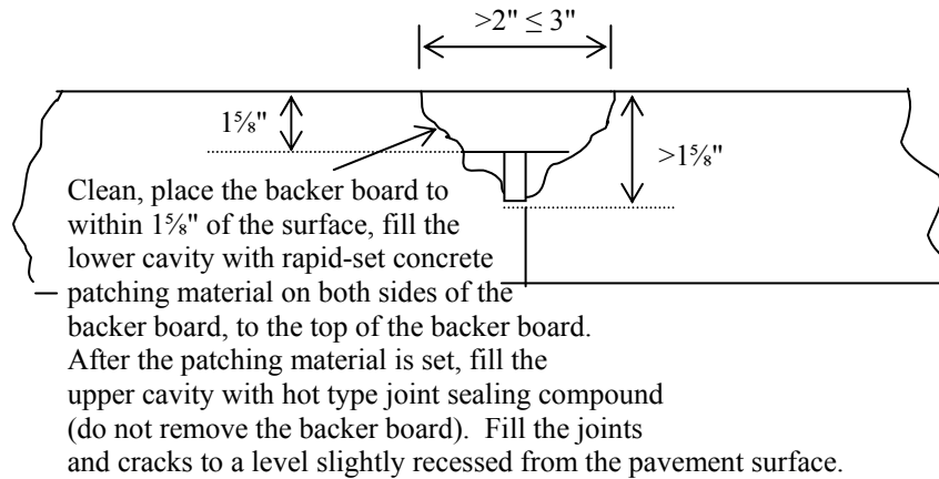
FIGURE 835-4: TYPE B, SEALING PCCP, SPALLED JOINTS AND CRACKS (>2" ≤ 3" wide, >1 5/8" deep)
